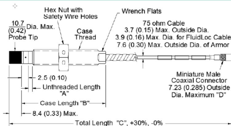
Figure 11: 3300 XL 11 mm Proximity probes, Standard Mount
