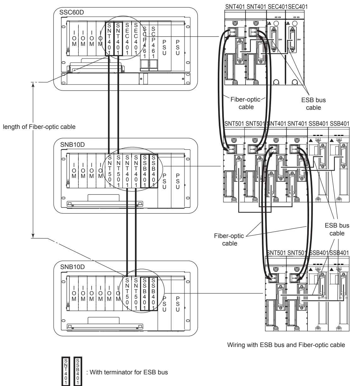
Figure Example of Chain Type Connection
