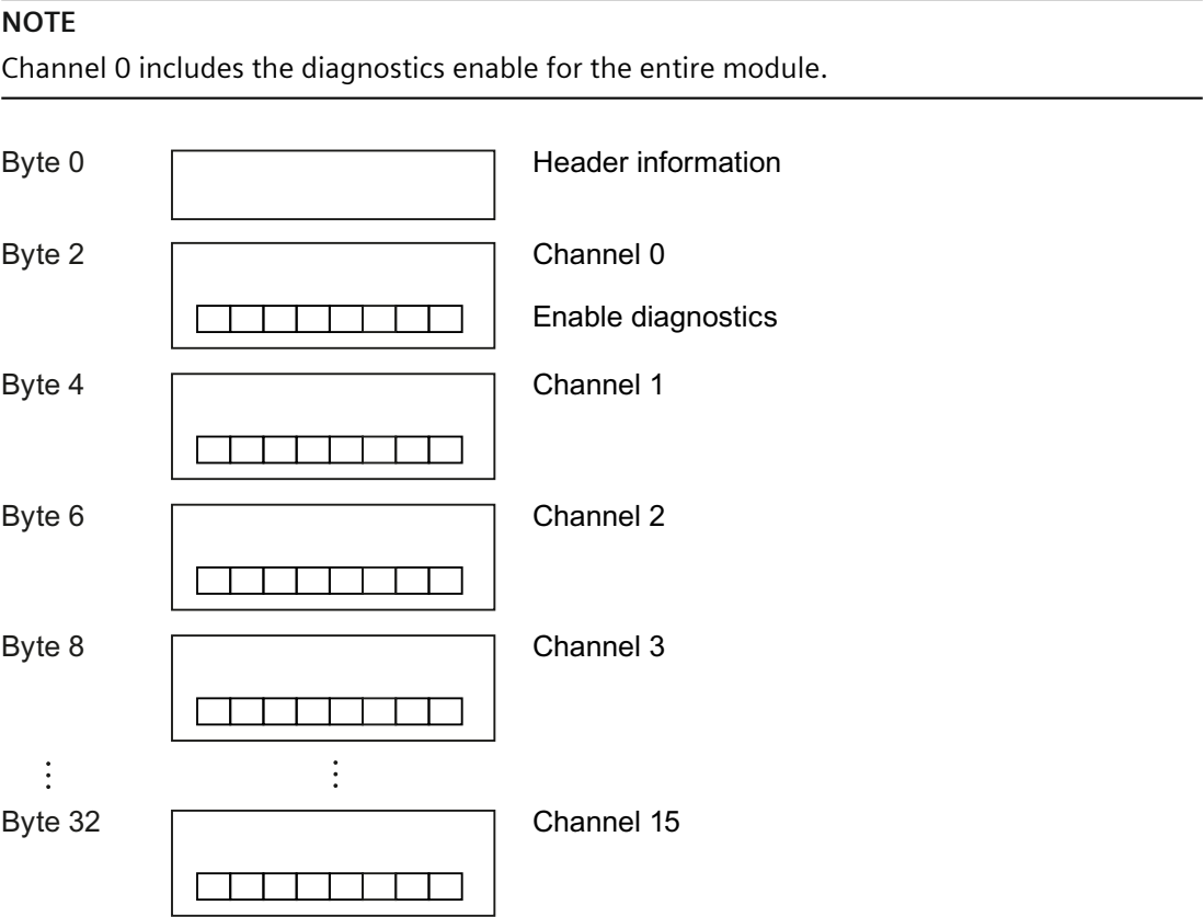
Figure A-1 Structure of data record 128
