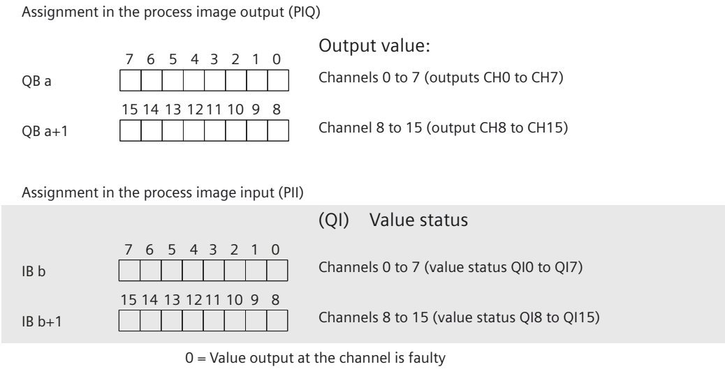
Figure 5-2 Address space for configuration as 16-channel DQ 16x24VDC/0.5A ST V0.0, QI
